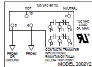
11 PIN SOCKET FOR MODEL 3002Y2
